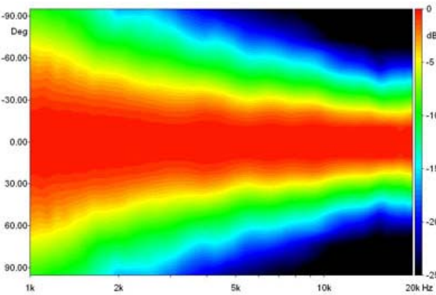
Vertical Beamwidth
